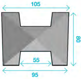
INTERMEDIATE POST (FOR PANELS)
