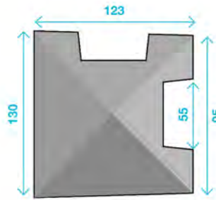
CORNER "L" SECTION POST (FOR PANELS)
