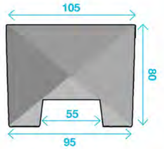
END "C" SECTION POST (FOR PANELS)
